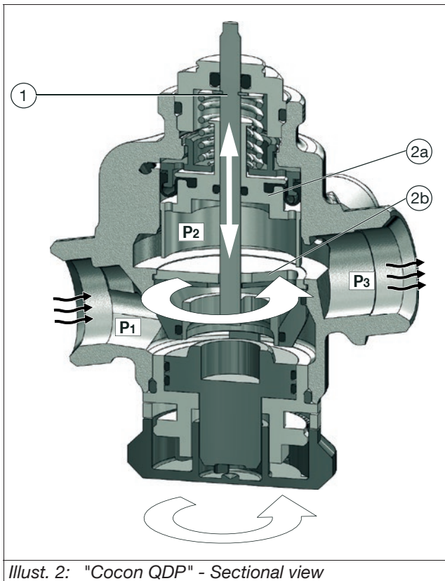
Illust. 2: "Cocon QDP" - Sectional view
