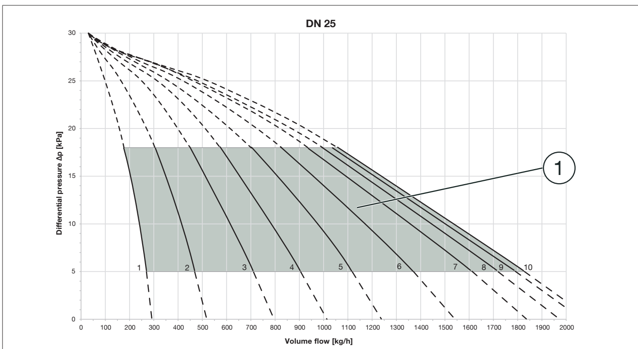
Illust. 9: Handwheel settings characteristic lines DN25
