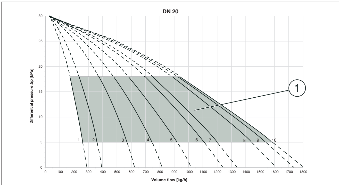
Illust. 8: Handwheel settings characteristic lines DN 20
