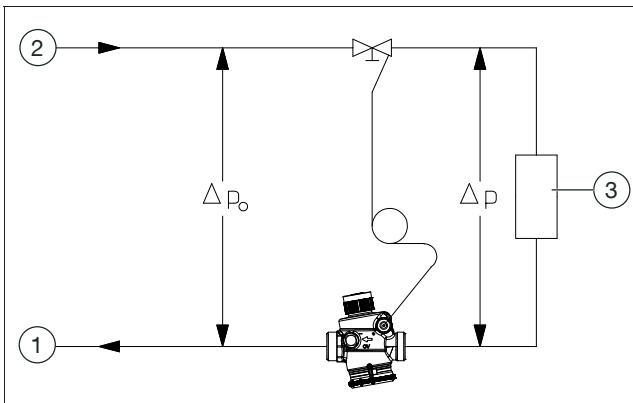
Illust. 4: Installation example
