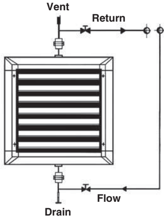
Horizontal discharge
